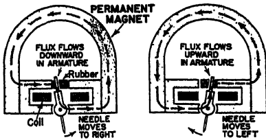
Operating principle of a magnetic phonograph pickup.
